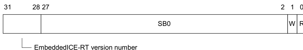
Figure 9-6 Domain Access Control Register
